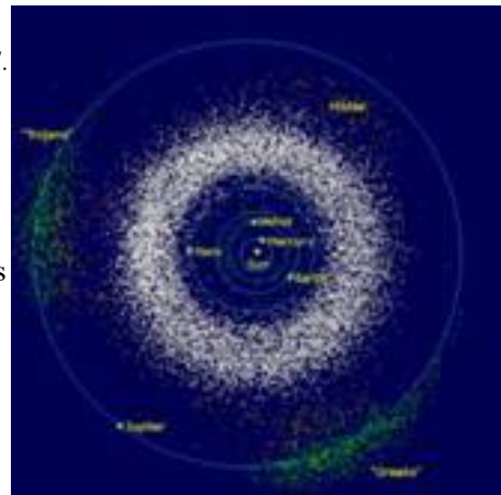
Fig. J.2.a Asteroid belt [Wikipedia.de].
